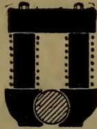
Diagram of magnetic circuit of Edison dynamo. Leakage coefficient 1.4.
